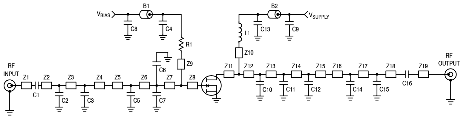
Figure 23. MMRF1021NT1 Broadband Reference Circuit Schematic — 760–860 MHz
