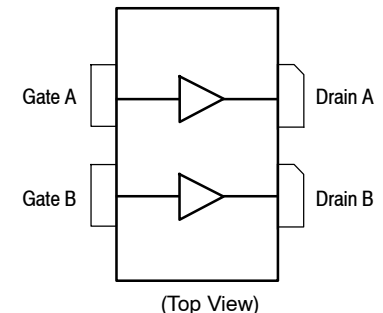
Figure 1. Pin Connections
