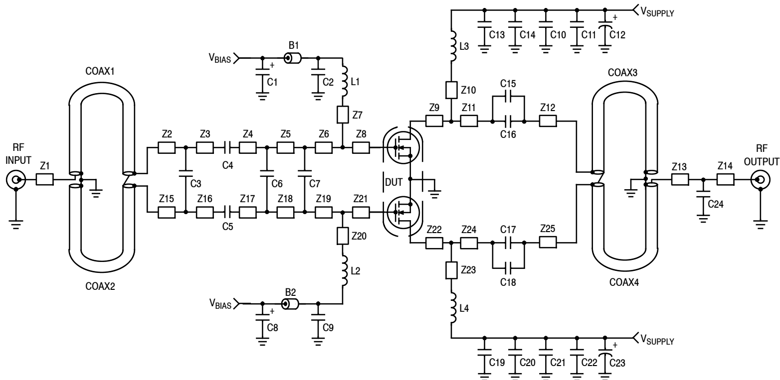
Figure 6. MMRF1305HR5(HSR5) Narrowband Test Circuit Schematic — 512 MHz
