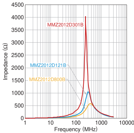
MMZ2012D series
