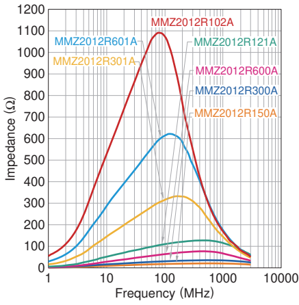
MMZ2012R series
