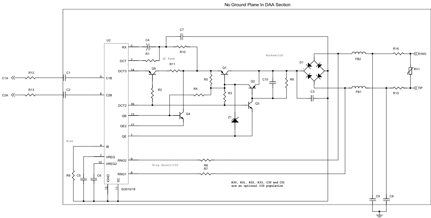
Figure 14. Si2457FT18-EVB Modem Board Page 2
