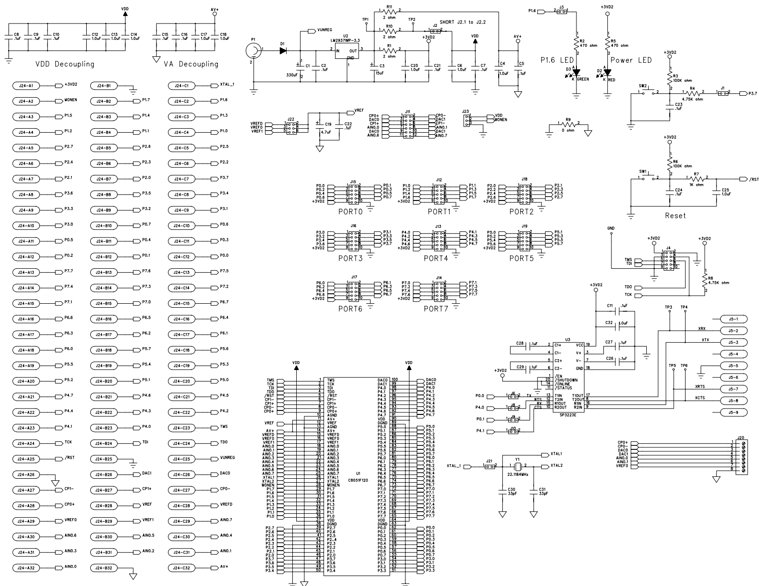
Figure 9. C8051F120 Target Board Schematic
