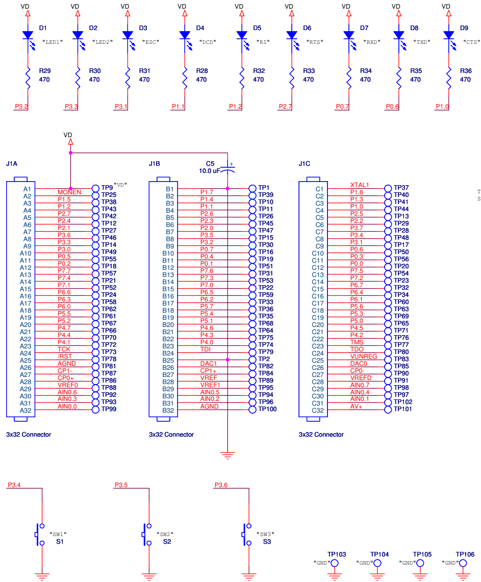
Figure 11. AB3 Modem Adapter Board Page 2
