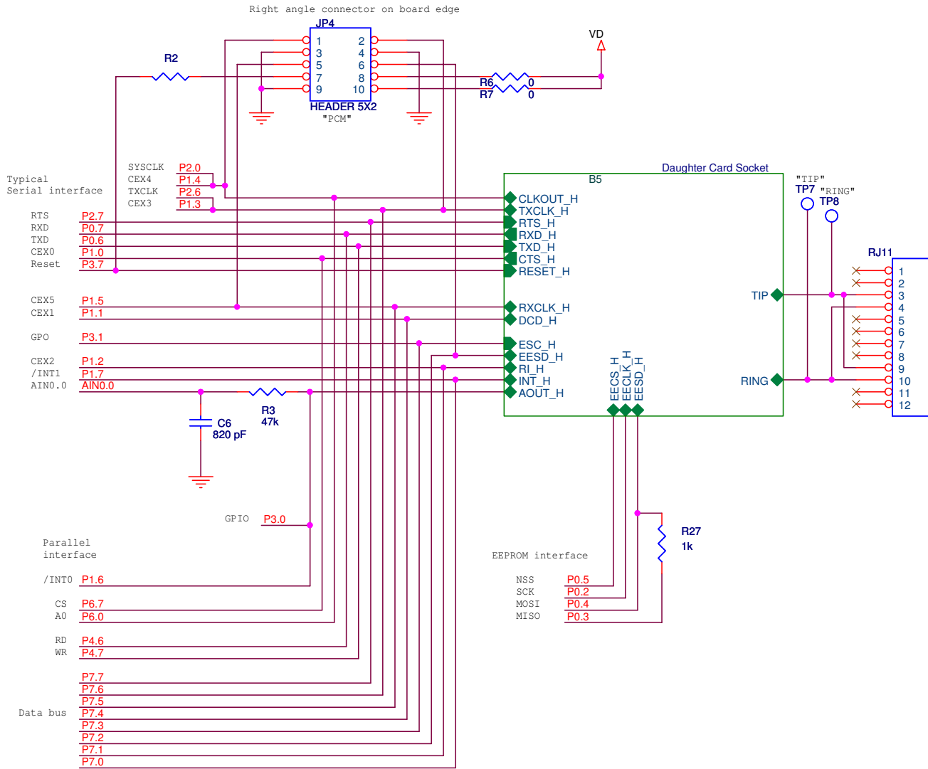
Figure 10. AB3 Modem Adapter Board Page 1
