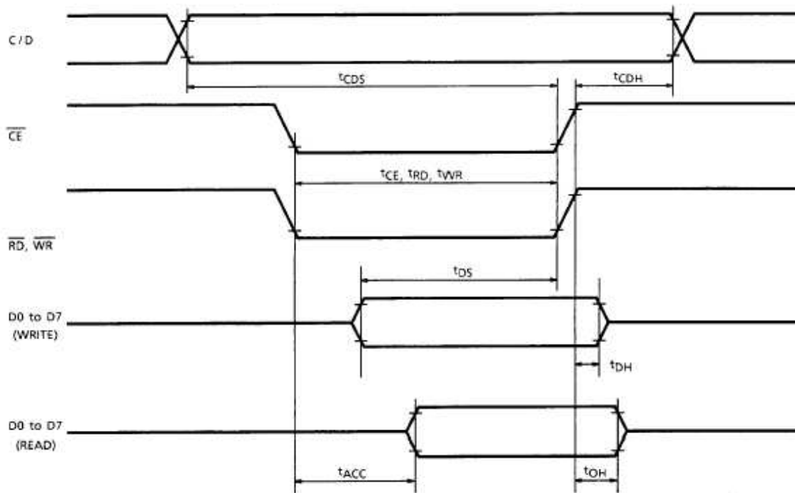
Figure 4: Timing Waveform
