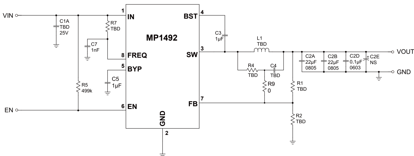
Figure 12—Typical Application Schematic with Low ESR Ceramic Capacitor
