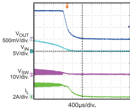
Shut Down Through VIN I_{OUT} = 2A
