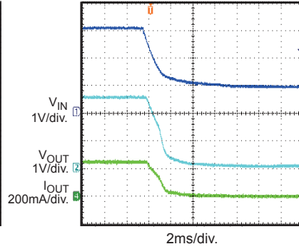
Input Power Shut Down with Resistive Load
