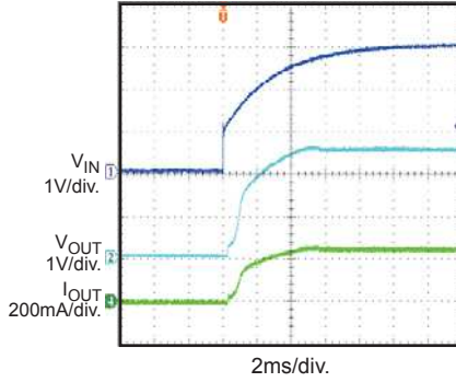
Input Power Start Up with Resistive Load
