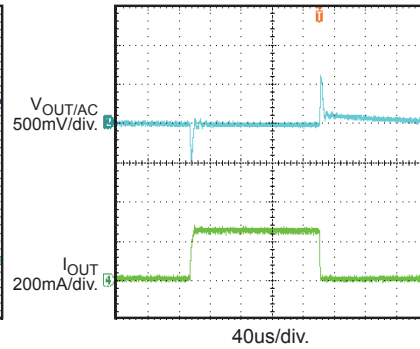
Load Transient with Resistive Load
