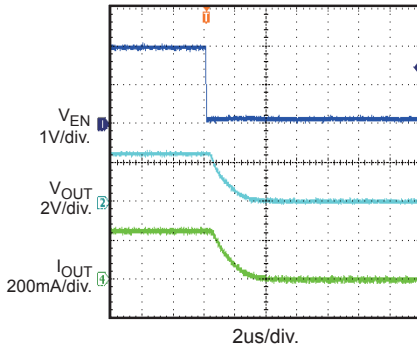
EN Shut Down with Resistive Load
