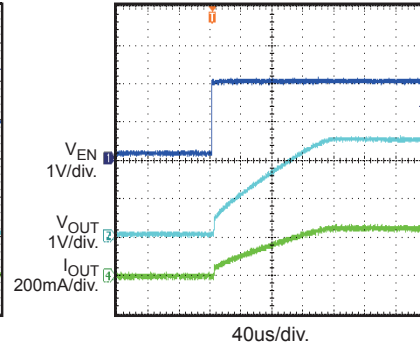
EN Start Up with Resistive Load
