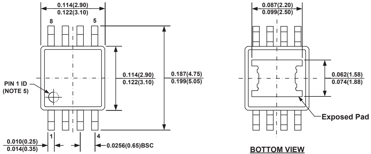
TOP VIEW
