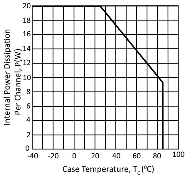
Figure 19: Power Derating
