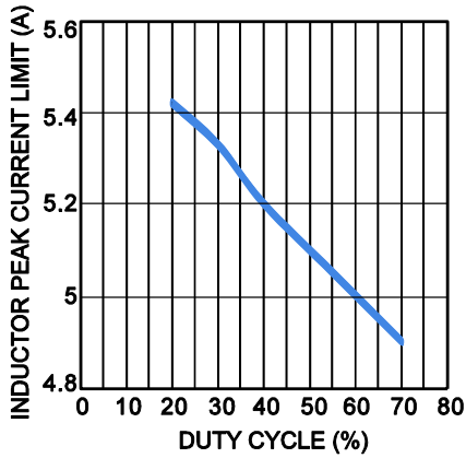
Inductor Peak Current Limit vs. Duty Cycle
