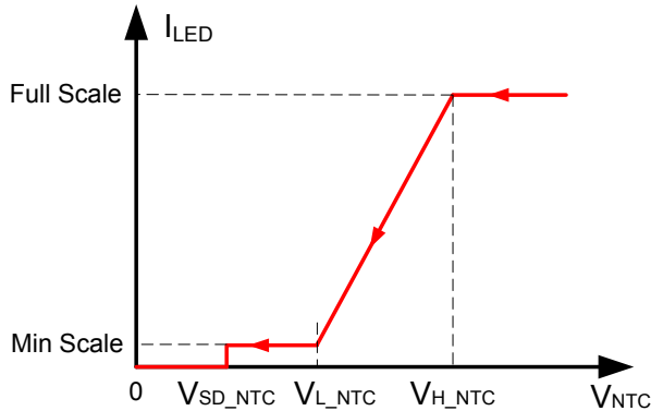
Figure 4: NTC Curve
