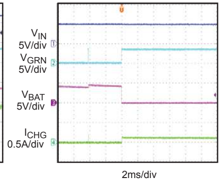
Short Circuit
