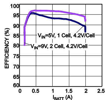
Efficiency Curve
