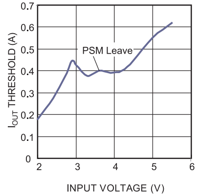
PSM to PWM Transition Threshold
