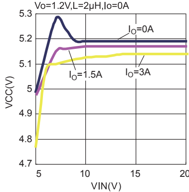
VCC vs. Input Voltage
