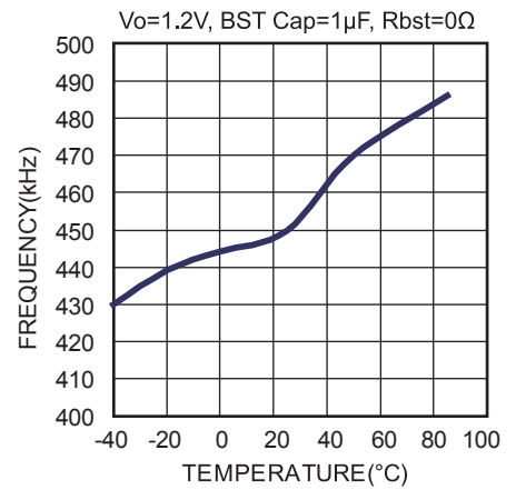
Fs vs. Temperature
