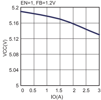
VCC vs. I o
