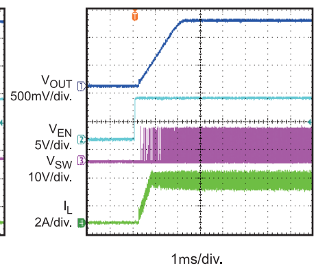
Start Up Through EN
