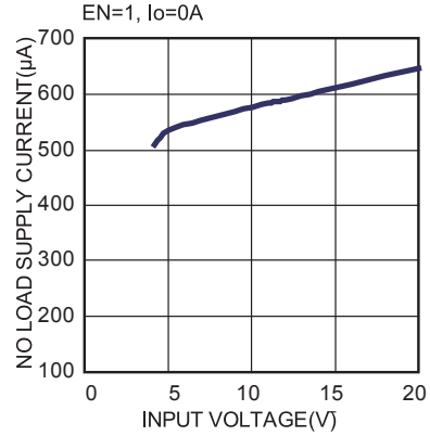
No Load Supply Current vs. Input Voltage
