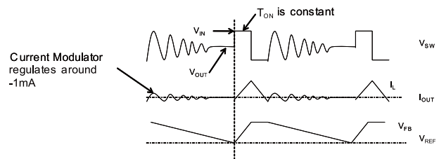
Figure 3: Light-Load Operation
