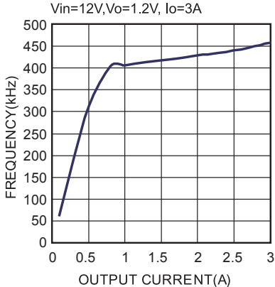
Fs vs. Output Current
