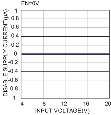
Disable Supply Current vs. Input Voltage
