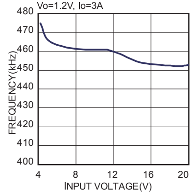
Fs vs. Input Voltage
