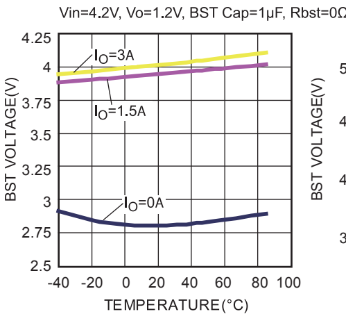
BST Voltage vs. Temperature
