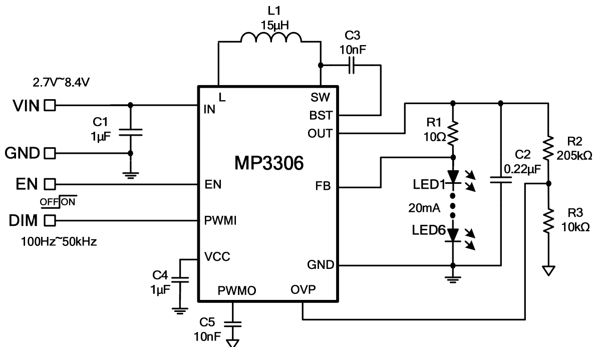
Figure 6— 6 LEDs in Series with PWM Dimming
