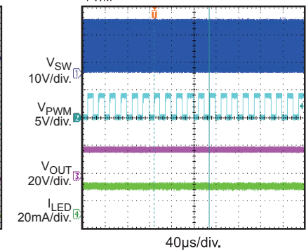
PWM Input Analog Dimming
