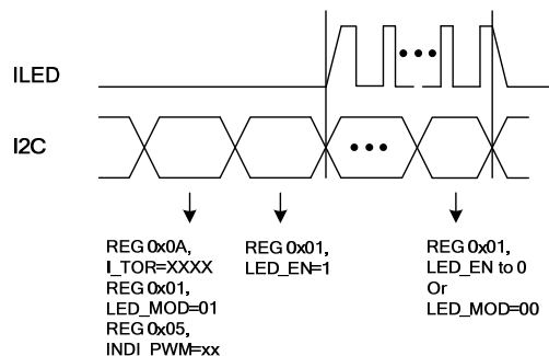
Figure 5: Indicator Mode
