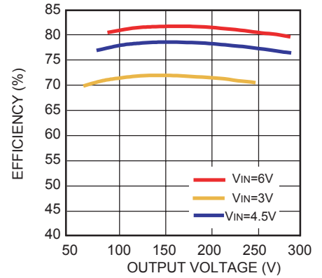
Efficiency at I_{SET}=2.5\text{A}
