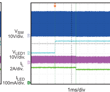
Short LED Protection Short channel LED1
