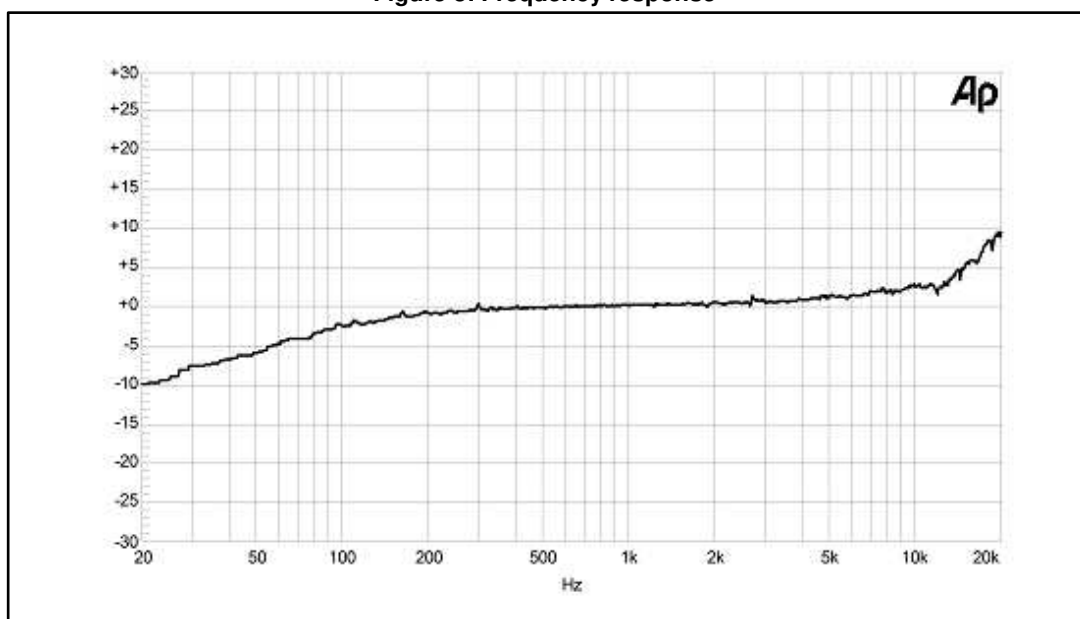
Figure 3: Frequency response
