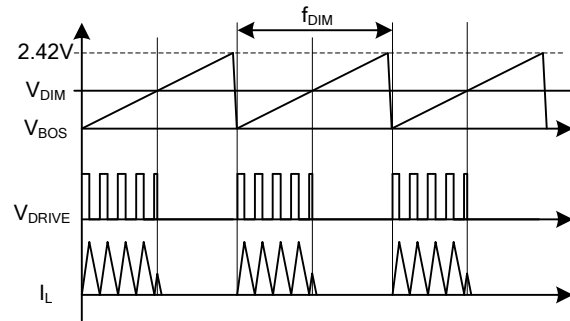
Figure 4: DC Burst Dimming
