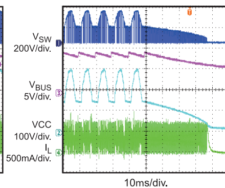
Power Down@220VAC
