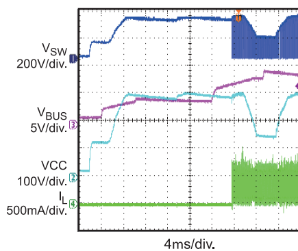
Power Up@220VAC
