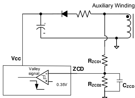
Figure 4: Zero-Current Detector
