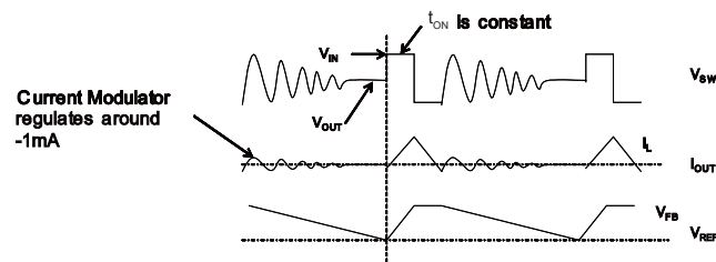
Figure 3: Light-Load Operation
