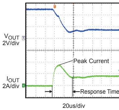
0.66Ω Load Connected to Enabled Device No Cdv/dt, No C OUT
