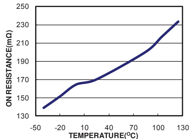
Bridge B LS On Resistance vs. Temperature VIN = 24V, IOUT = 1A
