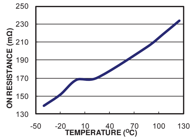
Bridge A LS On Resistance vs. Temperature VIN = 24V, IOUT = 1A
