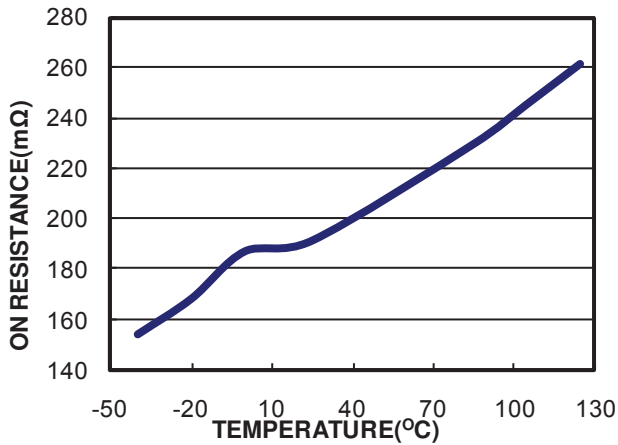
Bridge A HS On Resistance vs. Temperature VIN = 24V, IOUT = 1A
