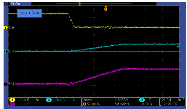
Figure 6: Switching with Resistance and Diode
