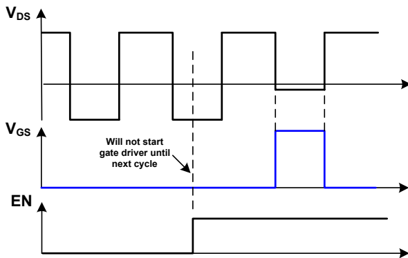
Figure 2: EN Control Scheme
