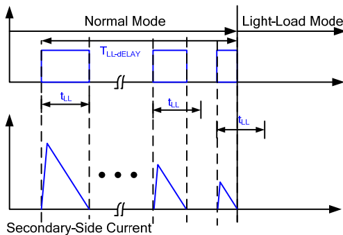
Figure 5: MP6906 Enters Light-Load Mode
