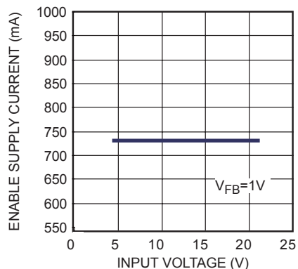
Enable Supply Current vs Input Voltage
