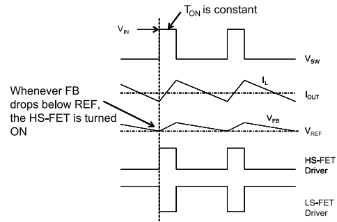
Figure 2: Heavy-Load Operation
