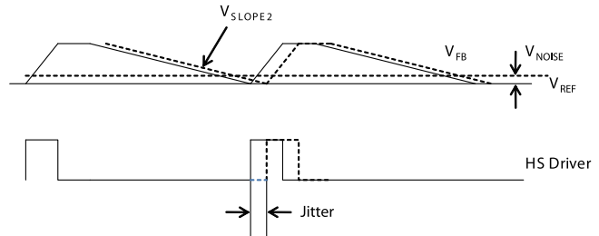
Figure 5: Skip-Mode Jitter
