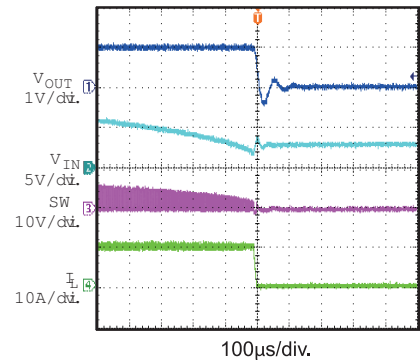
Shutdown Through I_{IN} I_{OUT}=10A
