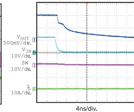
Shutdown Through I_{IN} I_{OUT}=0A
