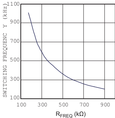
Switching Frequency vs. R_{FRQ}
