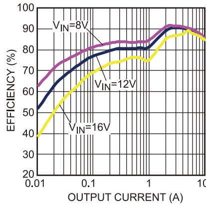
Figure 26 — Efficiency Curve
