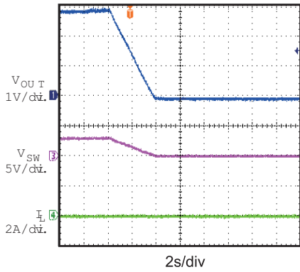
Thermal Shutdown I_{OUT} = 0A , V_{OUT} = 3V
