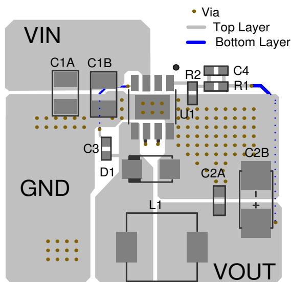
Figure 3: Recommended Layout
