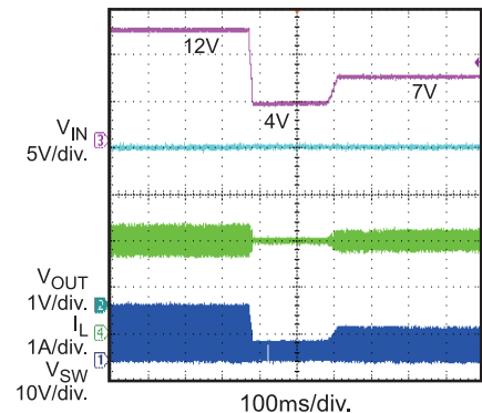
Cold-Crank V_{OUT}=3.3V , I_{OUT}=2A
