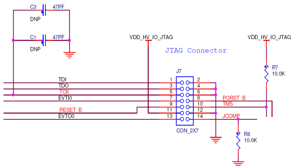
Figure 6. JTAG Interface
