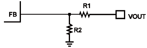
Figure 7. Feedback Network
