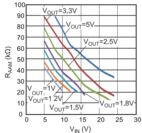
Figure 10. Recommended AAM Resistor Selection
