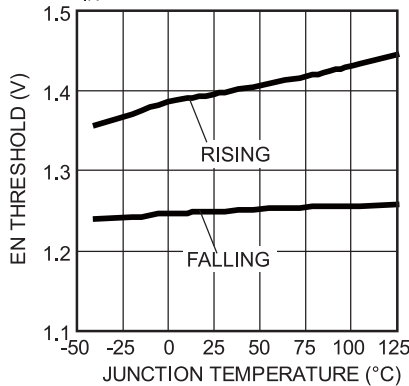
EN Threshold vs. Junction Temperature V_{IN}=12V
