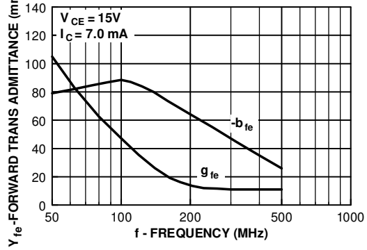
Forward Transfer Admittance vs Frequency
