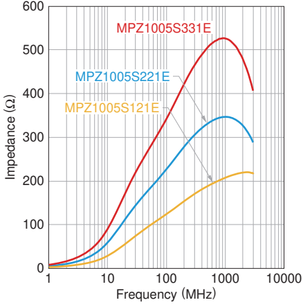
MPZ1005S-E series
