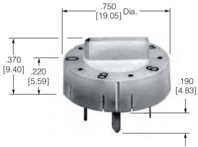
screwdriver/coin actuated Part Number 435005-1
