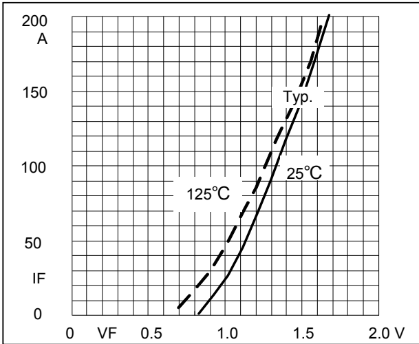
Fig1. Forward Characteristics
