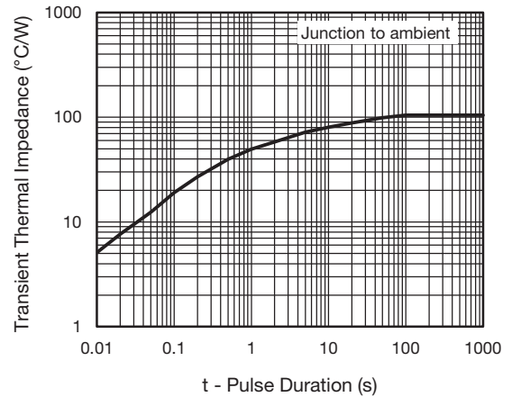
Fig. 7 - Thermal Resistance
