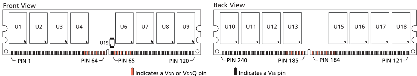
Figure 2: Pin Locations
