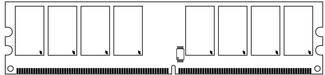
Figure 1: 240-Pin UDIMM (MO-237 R/C B and E)
