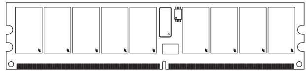
Figure 1: 240-Pin RDIMM (M O-237 R/C C-Non-Parity, R/C H-Parity)
