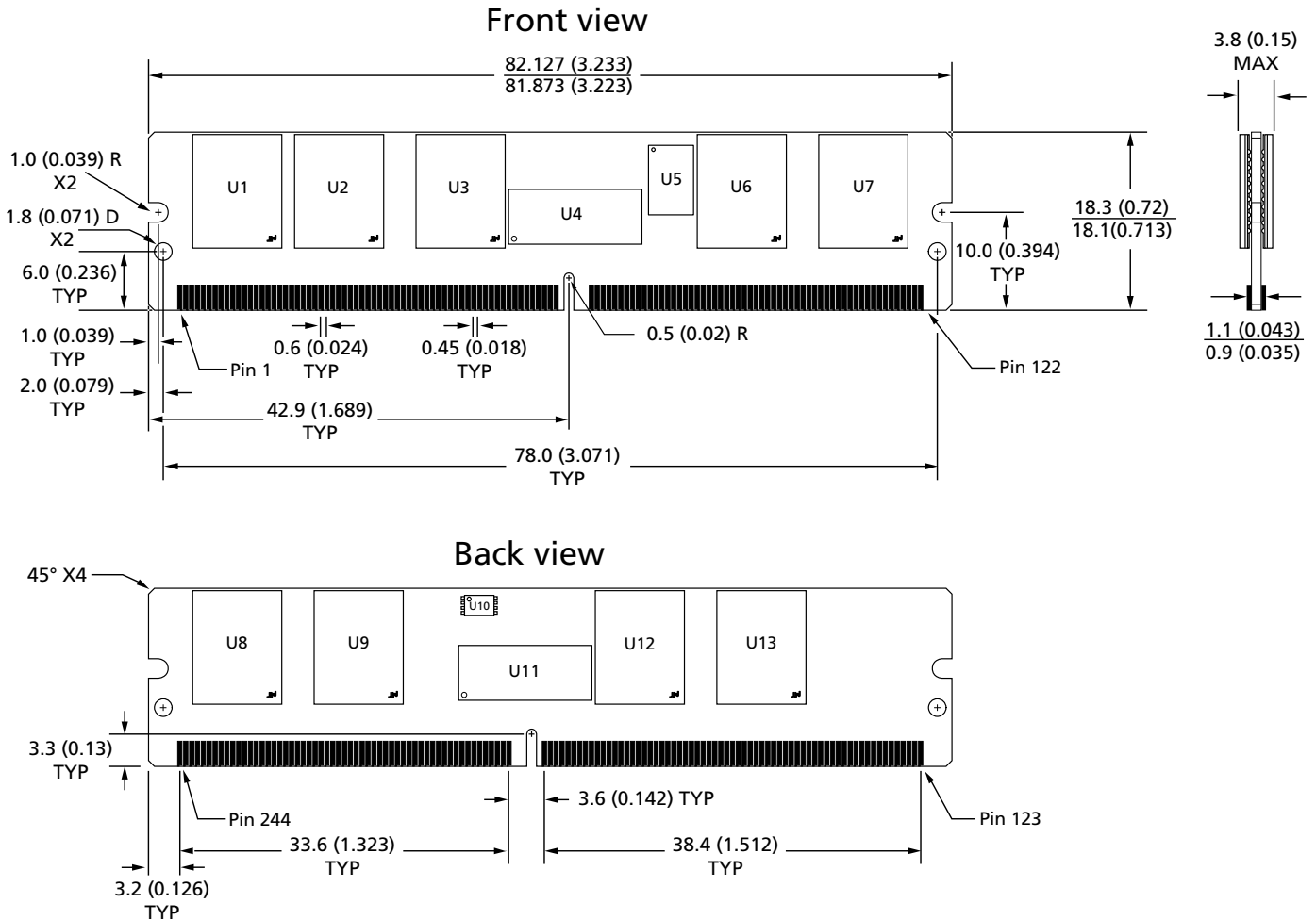
Figure 3: 244-Pin DDR2 VLP Mini-RDIMM
