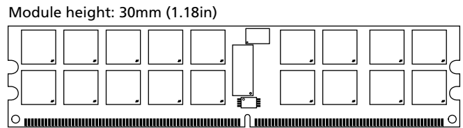
Figure 1: 240-Pin RDIMM (MO-237 R/C J – 2GB; R/C L – 4GB )
