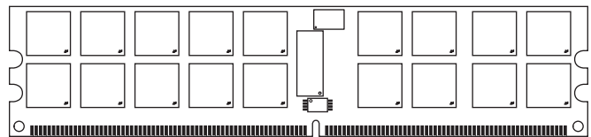
Figure 1: 240-Pin DIMM (M O-237 R/C L-4GB, R/C J-2GB)
