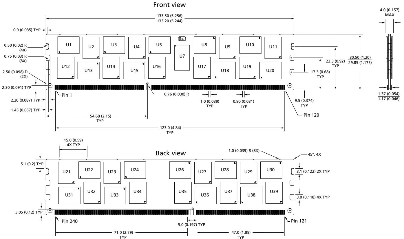
Figure 3: 240-Pin DDR3 RDIMM
